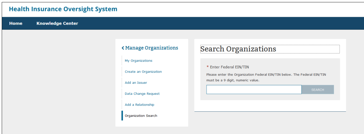
Figure 3-71: Organization Search
